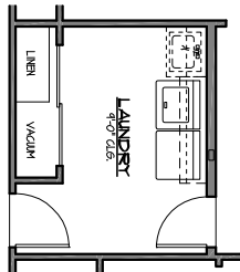
OPT. CLOSET I/O CABINETS AT LAUNDRY
