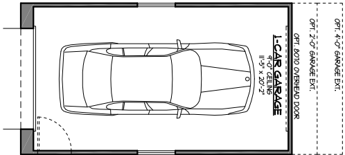
OPT. DETACHED 1-CAR GARAGE
