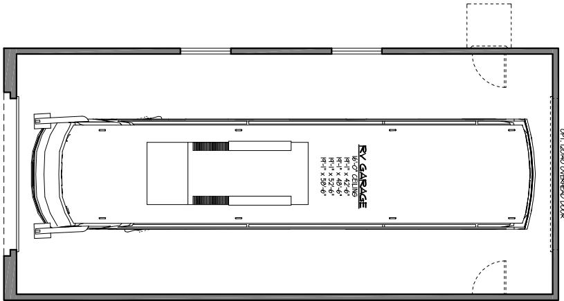
OPTIONAL DETACHED RV GARAGE
